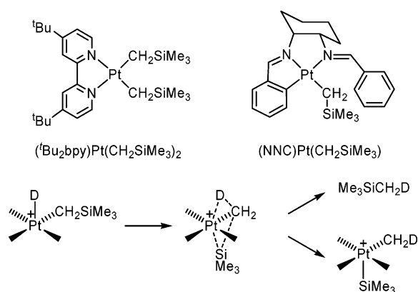
Scheme 57
