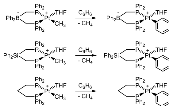
Scheme 35
