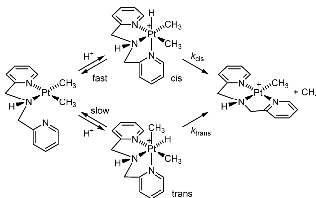
Scheme 57
