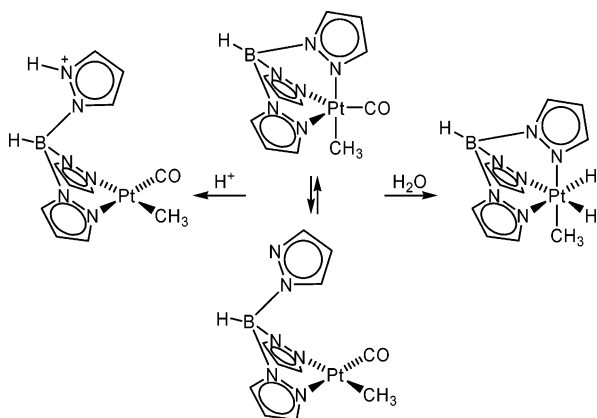
Scheme 74
