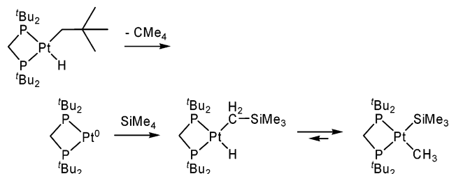
Scheme 23
