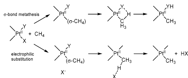
Scheme 17
