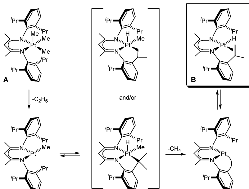
Scheme 90
